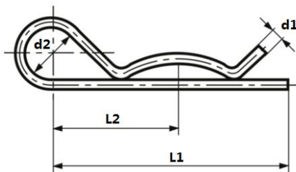
SNAP PIN (DIN 11024)
